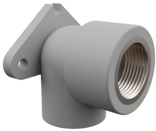
AQUASYSTEM Female Backplate Elbow Type 3 BSPP-G PP-R
